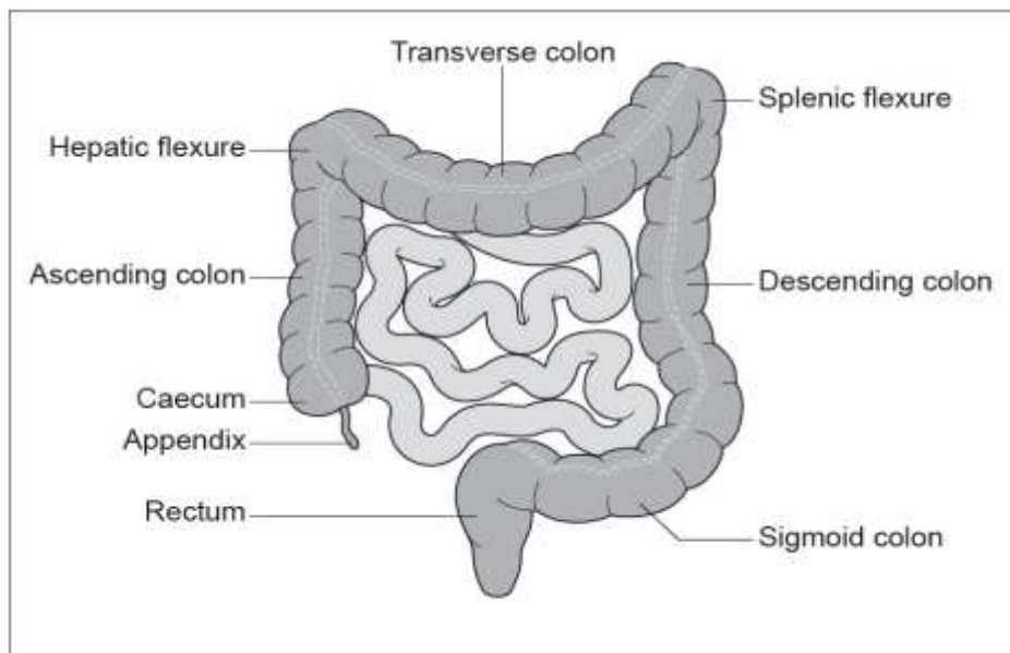
Figure 1: The colon
